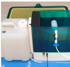
<Direct type>
